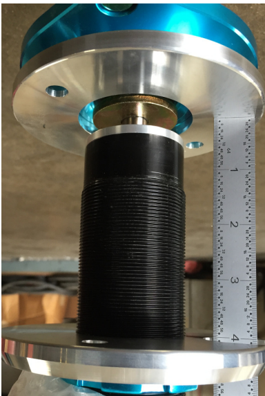
6. Loosely assemble upper strut mount and bag assembly. Then compress the shock and adjust lower perch so there is 4" between your bag plates.
