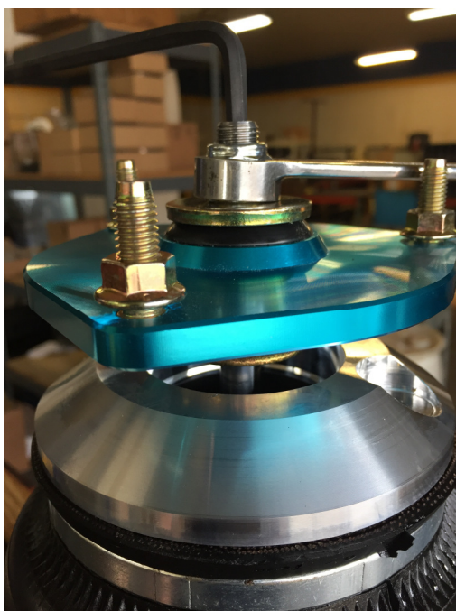
14. Tighten upper strut nut
