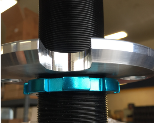
5. Loosely thread down lower bag plate.
